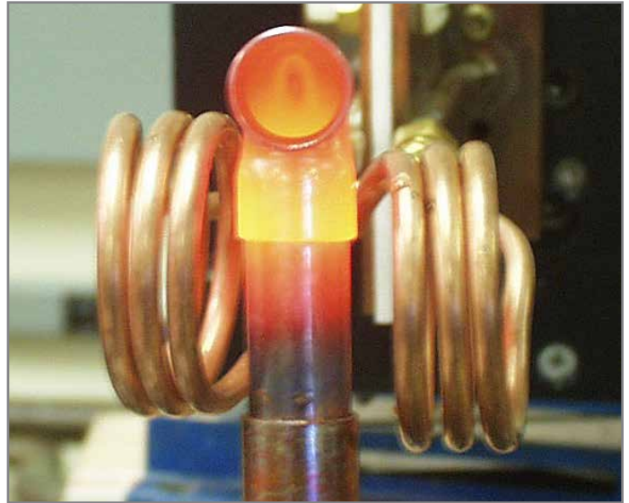
Replacing torch brazing on a copper elbow to copper pipe using a split helix coil. 7 kW at 190 kHz for 90 seconds to 760°C (1400°F).
